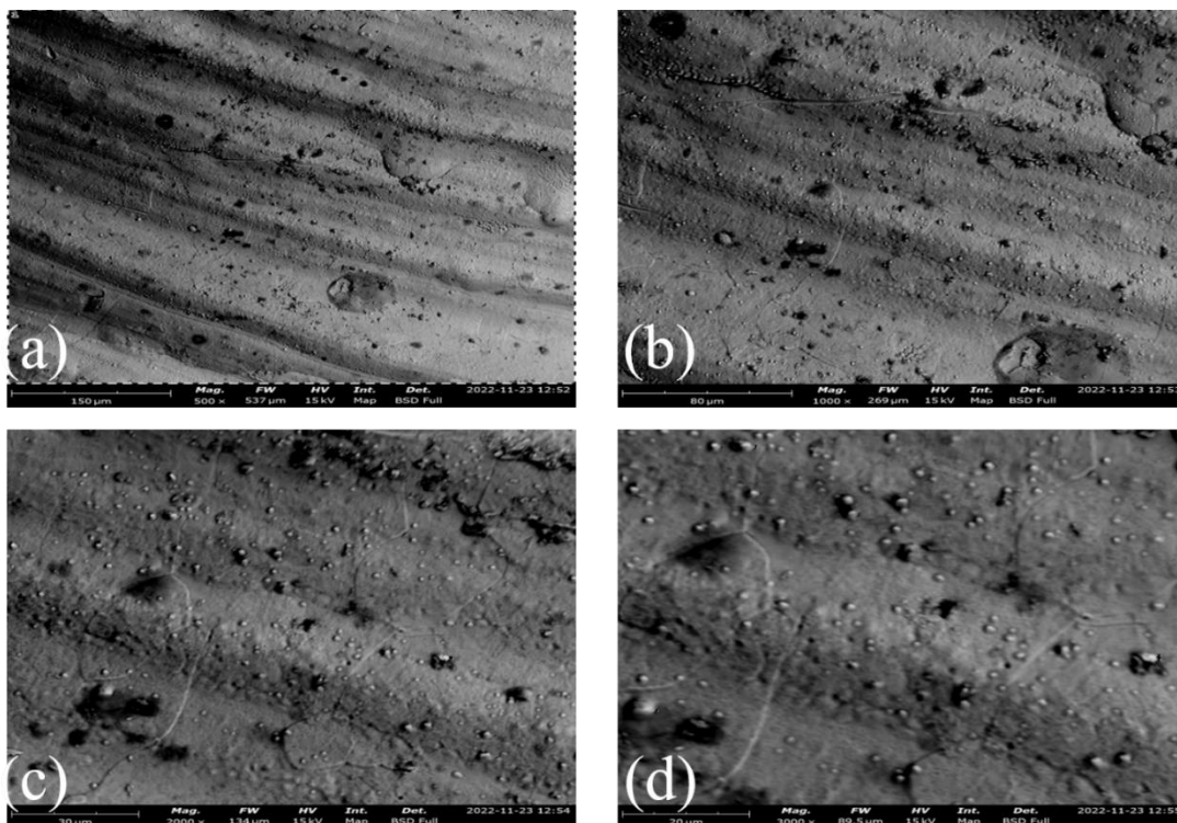
Figure 1: Microstructure of weld zone (a) 500x, (b) 1000x, (c) 2000x and (d) 3000x
